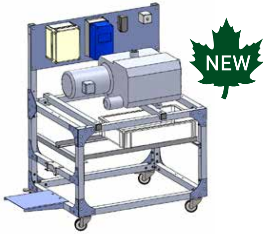
Adjustable cart for vacuum pump L25-L40-L63-L100 6660100
